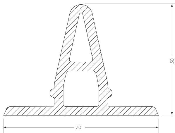
RENOLIT ALKORDESIGN profiel X-Large
