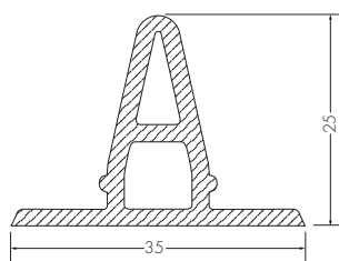
RENOLIT ALKORDESIGN profiel Large
