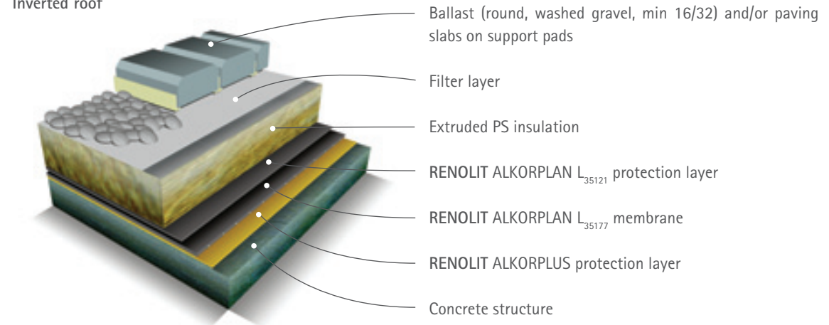
Inverted roof
