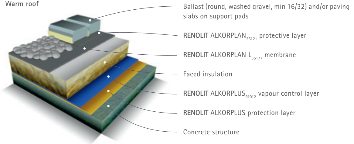
Warm roof
