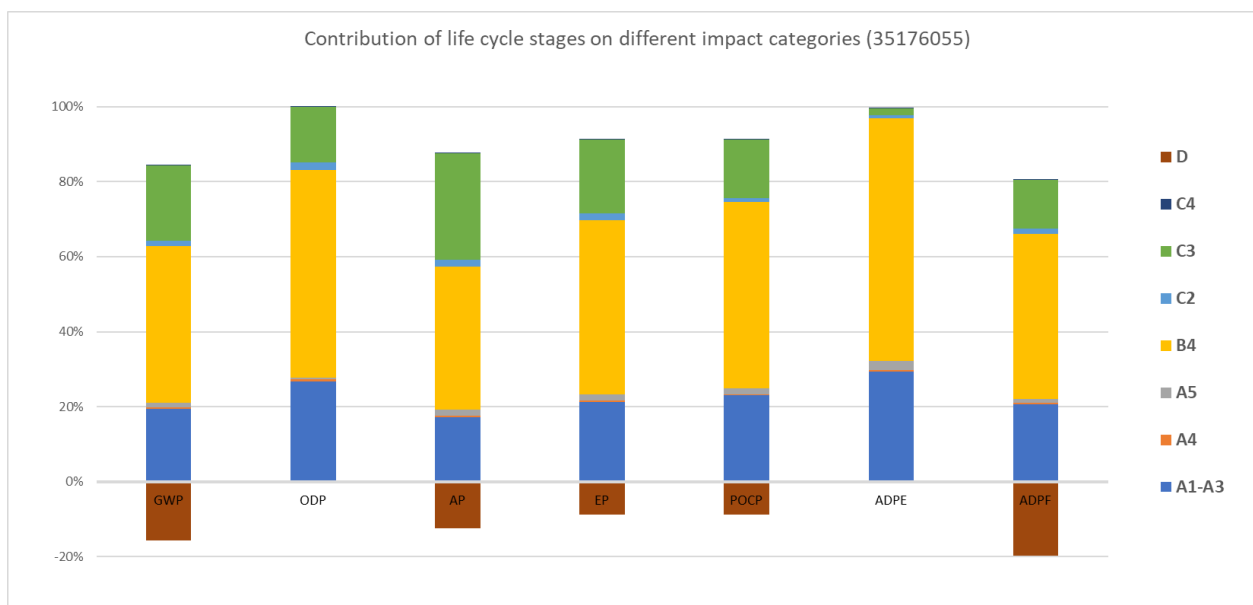
Figure 2: Contribution of the different life cycle stages to the environmental impact of one m 2 of Alkorplan F.
