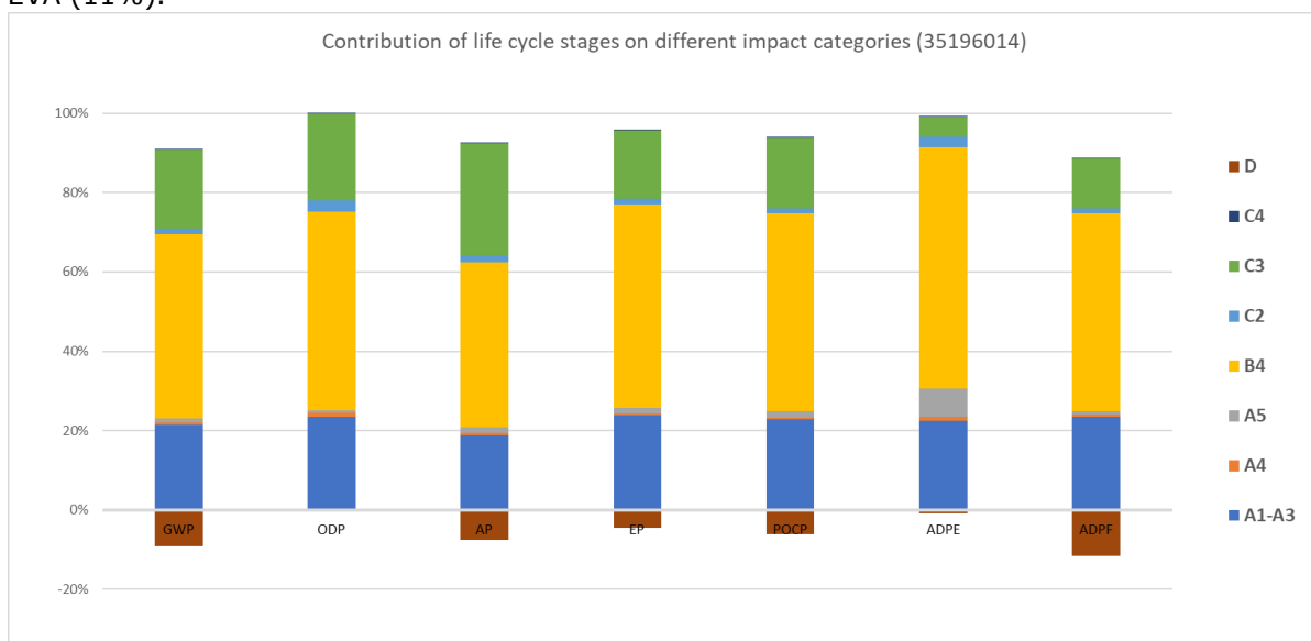
Figure 2: Contribution of the different life cycle stages to the environmental impact of one m 2 of Alkotec F.
